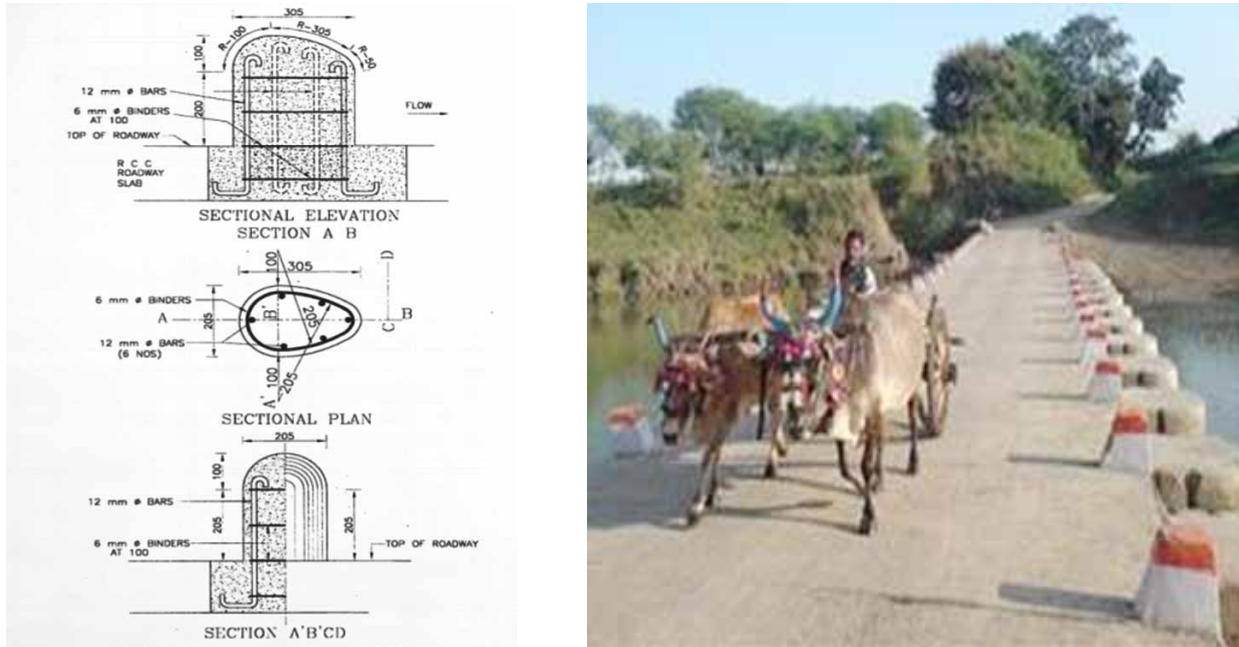
Fig. 14.10: Guard Posts as recommended by IRC: SP: 82 – 20
