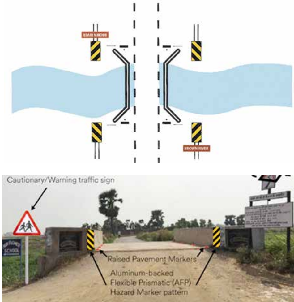
Fig. 14.9: Hazard Markers at Narrow Culvert
