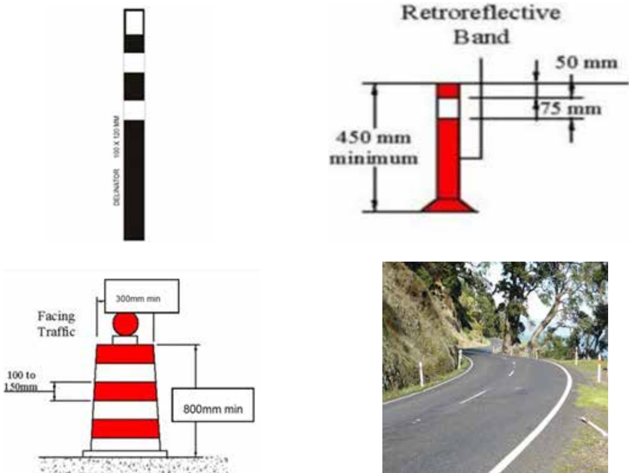
Fig. 14.7: Road Delineators
