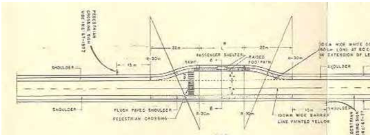
Fig. 14.4: Typical Layout for Bus Bays
