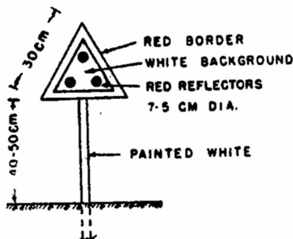
Fig. 14.11: Object Markers as per IRC: 79 – 1981
