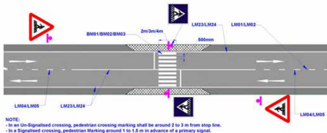
Fig. 14.6: Pedestrian crossing Markings on Rural Roads.
