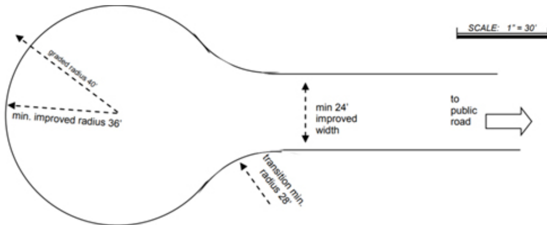
Fig. 14.3: Suggestive Layout for Space for Turning of Vehicles at the End of Rural Road
